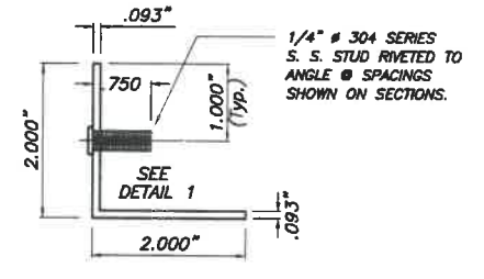
9 STUDDED ANGLE SCALE: 3/8" = 1"
