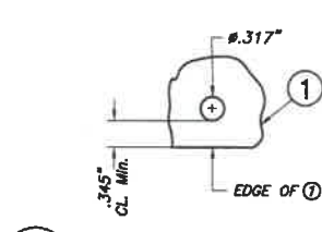
10A ROUND HOLE AT PANEL (OPTION TO 10)
